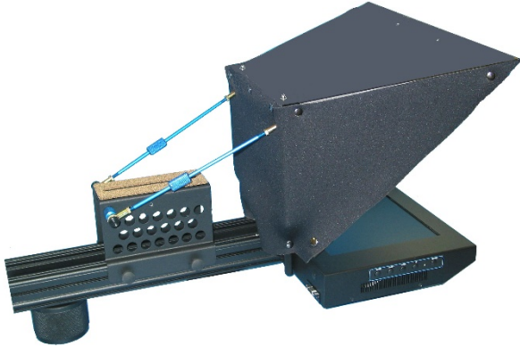
19B Prompter with wide angle beamsplitter and dual outrigger dynamic suspension and tensioning arms
