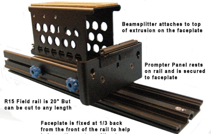
Ultra High Camera Riser puts the lens in the middle of the Beamsplitter
