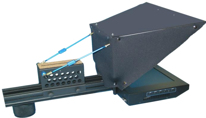
15V-ST with Ultra High Riser Camera Mount for Mini-DV Cameras, stabilized and dampened ST Hood and Beamsplitter
