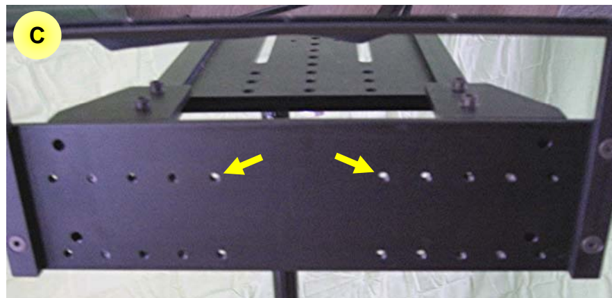
C Use a 1/4" drill bit to clear the threads from the two top centermost holes in the backplate – these are the mounting holes for the new LCD display.
